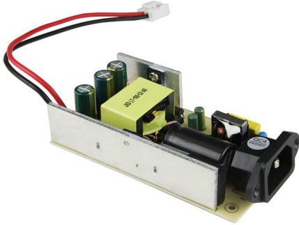
100W/52V Open Frame Power Supply
